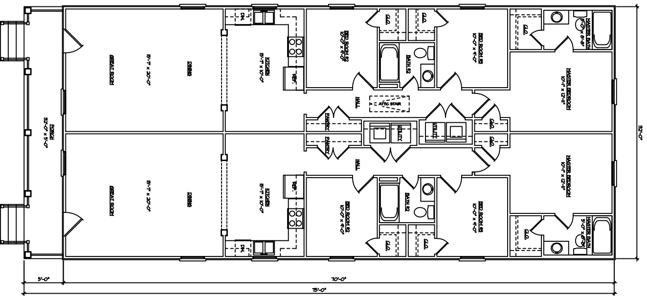
FIRST FLOOR PLAN SCALE: 1/4" = 1'-0"
